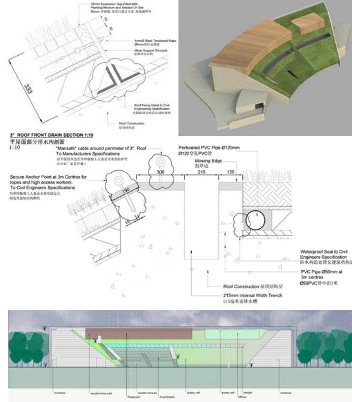
Milano Triennale, Shanghai, China Client: La Triennale di Milano Green Roof Construction Details
